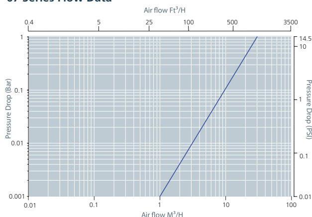
67 Series Flow Data
